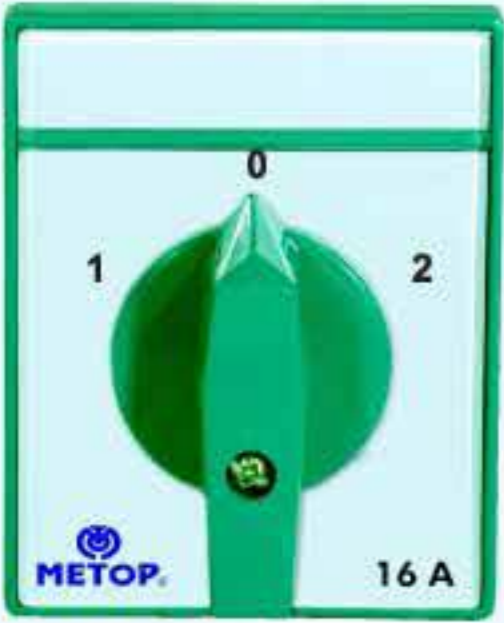
MT1197 Çift Devirli Motor Şalteri (Dahlender) Double Speed Motor Switch (Seperate Windings) (1-0-2) A 440
